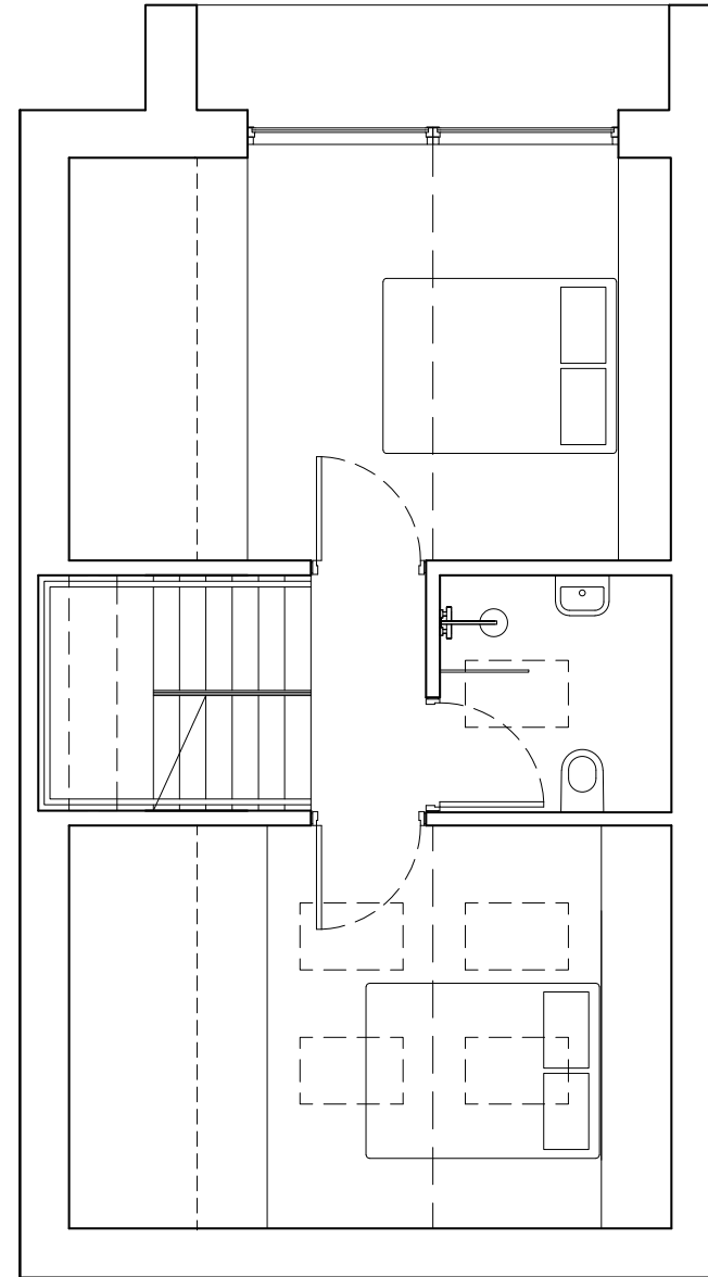
alternative second floor layout to provide a 4th bedroom
